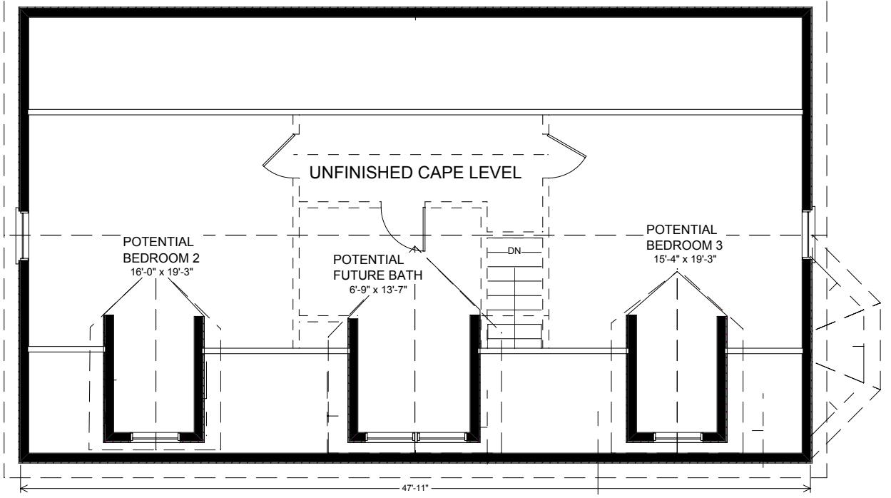
THE BAR HARBOR - 27'6" x 48'
