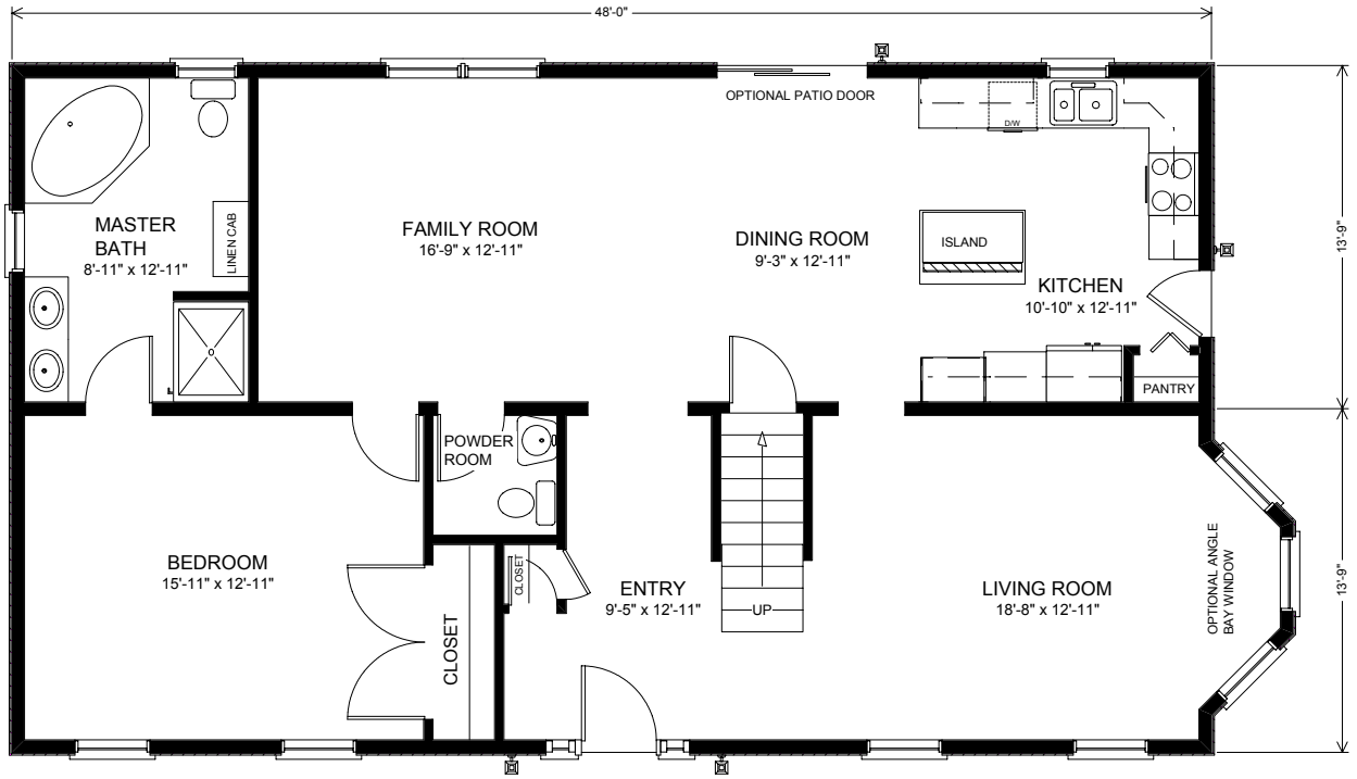
THE BAR HARBOR - 27'6" x 48'
